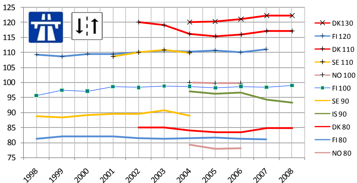
Fig.10: Development in mean speed of light vehicles on motorways and rural roads 1998-2008.
